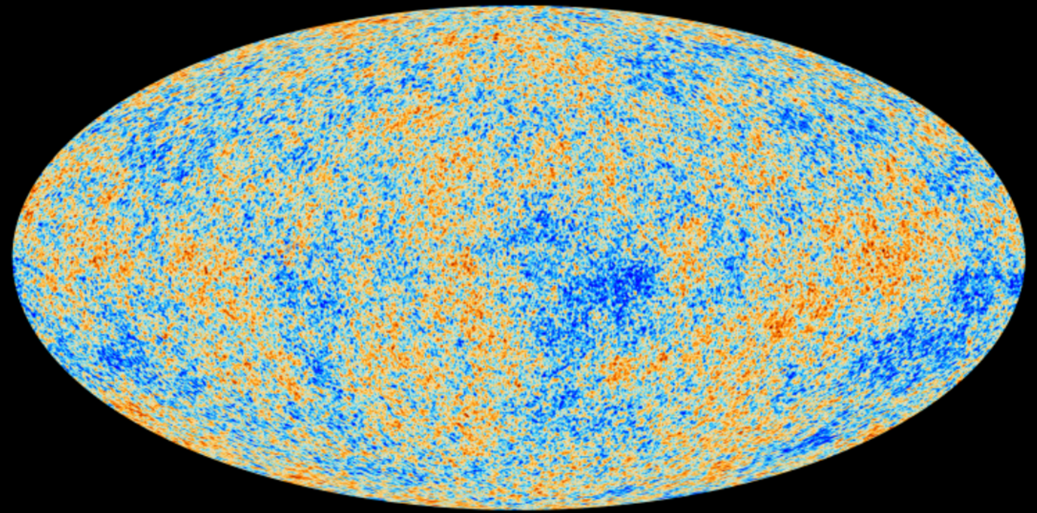
Cosmic background radiation
